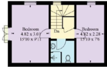
Annex 2 - First Floor
